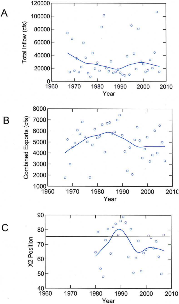
Figure 20. Trends in average spring (Apr-Jun) total delta inflow (A), combined SWP /CVP exports (B), and X2 position (C), 1967-2007, except for (C), which was 1980-2007. A LOWESS line was plotted through points to show general trend. The horizontal line in (C) at 75 km represents the location of Chipps Island.
